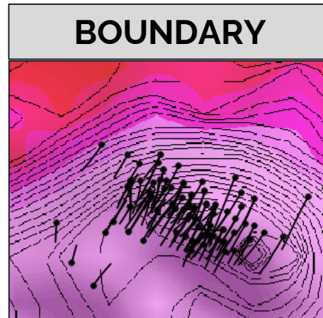
(Peak: 2.5 mGal)
